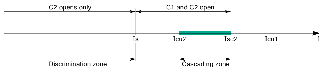
fig. 7: The principle of cascading between 2 circuit breakers, breaker C2 whose breaking capacity I_{cu2} is less than the three-phase short-circuit current at its terminals ( I_{sc2} ), is protected or assisted by breaker C1.
