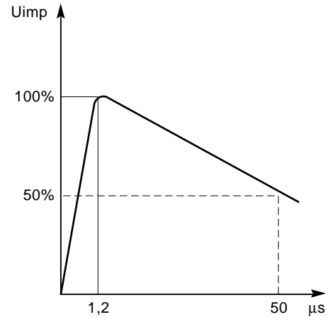
fig. 10: impulse wave for industrial circuit breakers 1.2/50 \mu\text{s} .
