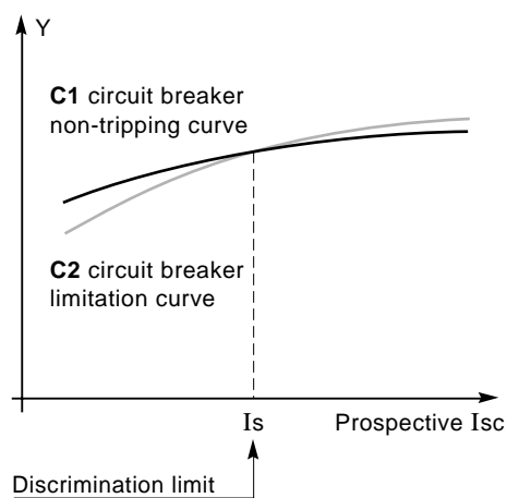
fig. 7: The principle of cascading between 2 circuit breakers, breaker C2 whose breaking capacity I_{cu2} is less than the three-phase short-circuit current at its terminals ( I_{sc2} ), is protected or assisted by breaker C1.
