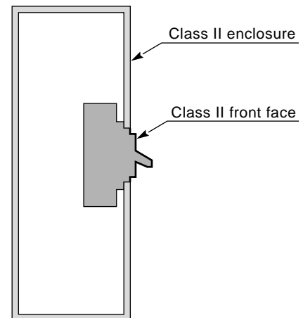
fig. 13: Class II equipment with circuit breaker having a class II front face.
