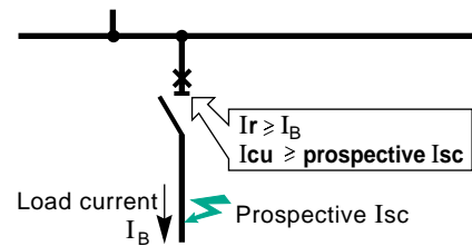
fig. 22: Basic parameter governing the selection of an outgoing circuit breaker.
