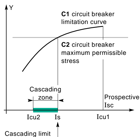
fig. 7: The principle of cascading between 2 circuit breakers, breaker C2 whose breaking capacity I_{cu2} is less than the three-phase short-circuit current at its terminals ( I_{sc2} ), is protected or assisted by breaker C1.
