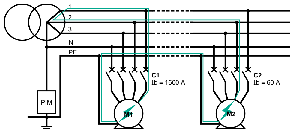
fig. 5: Example of « double fault » current breaking in an installation using the IT earthing system. The difference in ratings between two circuit breakers (C1 and C2) means that only one (C2) may be in a position to eliminate the fault with a single pole under phase-to-phase voltage.
