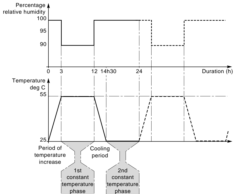
fig. 15: Test cycle for humidity/heat endurance, repeated over 28 consecutive days.
