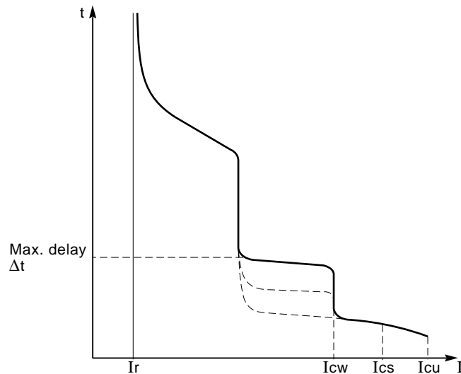
fig. 4: Additional test for category B circuit breakers.
