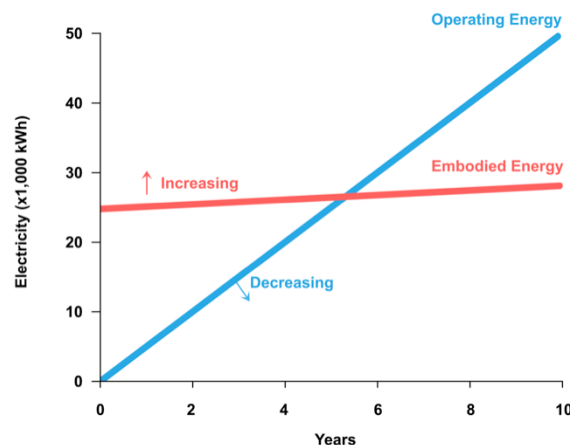
Embodied v. Operating Energy For A Cellular Base Station
