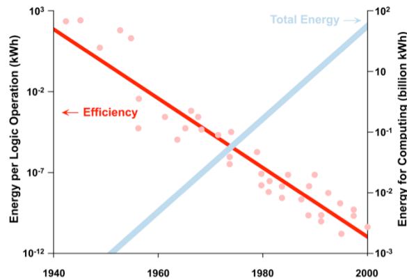
Computing Energy Efficiency v. Computing Energy Consumption
