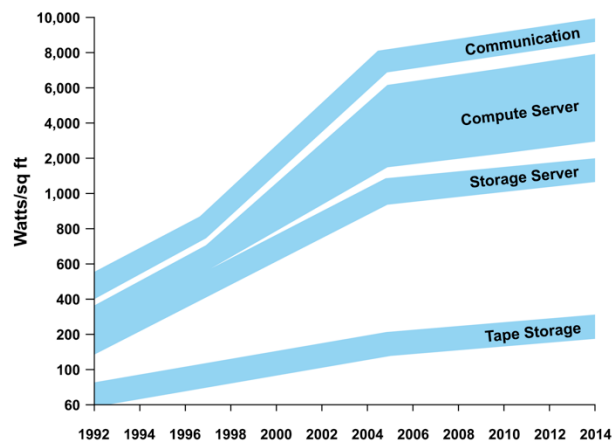
Global Data Center Power Trends Power of compute equipment by year of product introduction.
