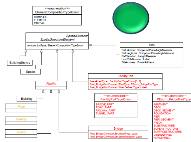
Figure 7 Spatial structure concepts for Bridge model.
