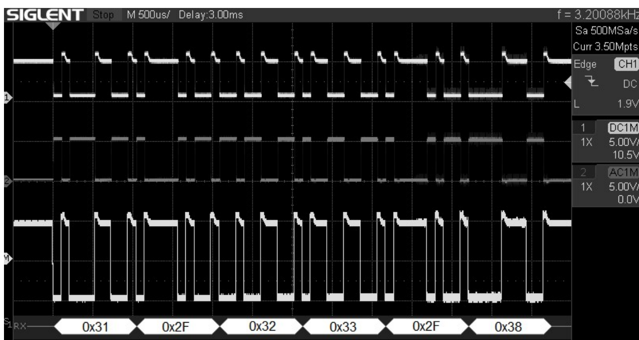
Figure 12 : trame RS485
