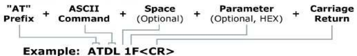
Figure 2-08. Syntax for sending AT Commands
