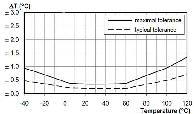
Figure 3 Maximal tolerance for temperature sensor in °C.
